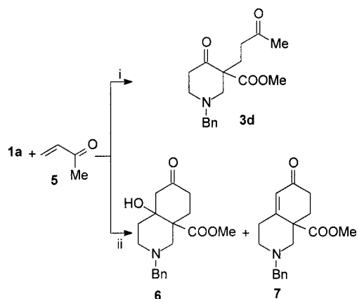
Scheme 2. Reagents and conditions: i, Dowex 66 (100%), MeOH, room temp., 120 h, 92%. ii, Dowex 550A (300%), EtOH, room temp., 120 h, then reflux, 6 h, 80%
