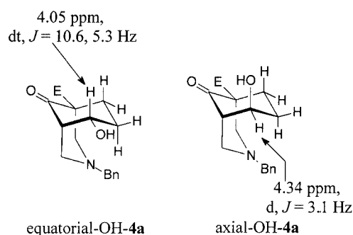
Figure 1. 1 H observations for 4a axial-OH and equatorial-OH (E = COOMe)
