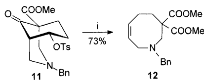
Scheme 5. Reagents and conditions: i, DBU (1.5 equiv.), MeOH, reflux, 4 h
